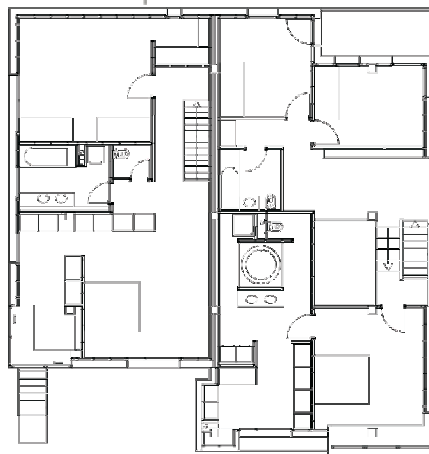
level +0.34
